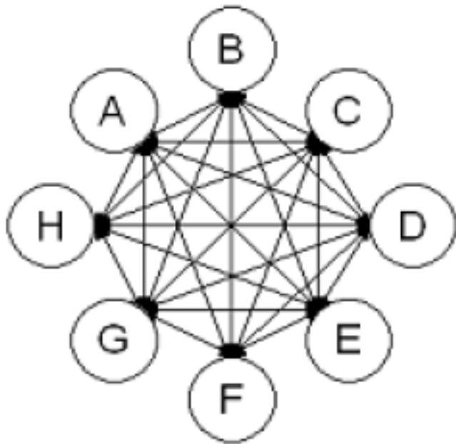
Figure 3.9 Peer-2-peer model
